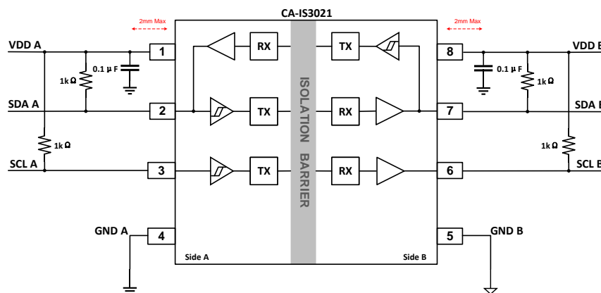
Figure. 10-2 The CA-IS3021 typical application circuit
