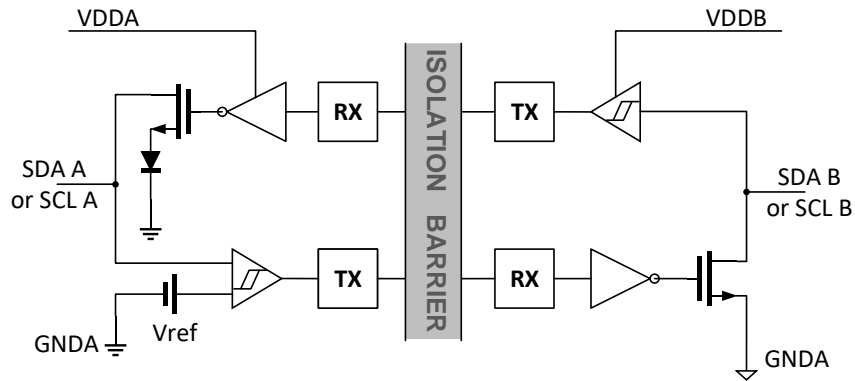
CA-IS302x functional block diagram
