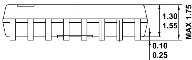
BOTTOM VIEW
