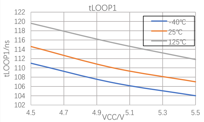
Figure 7-9 Loop Delay, Recessive to Dominant
