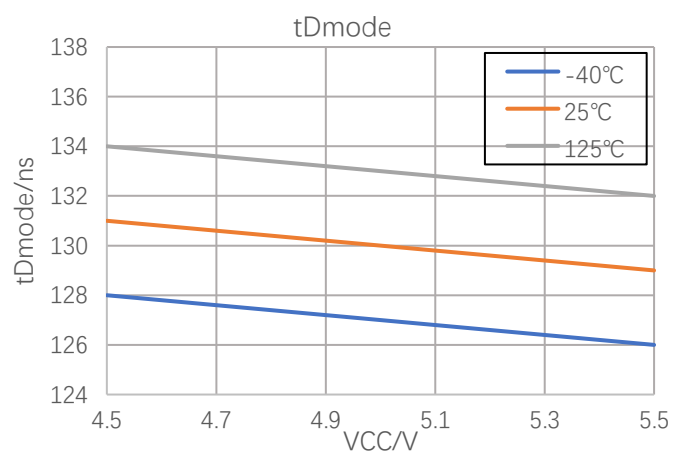
Figure 7-11 Mode Change Time
