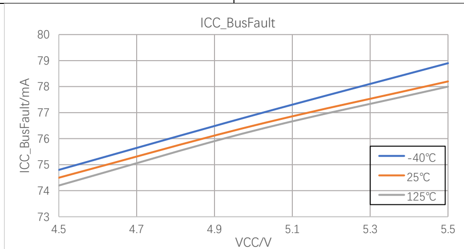
Figure 7-5 Bus Fault Current
