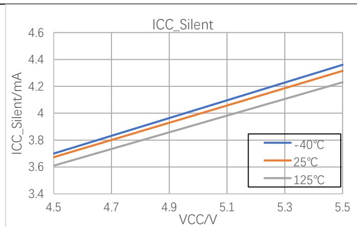
Figure 7-1 Supply Current @ Silent Mode
