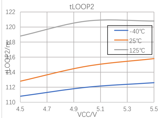
Figure 7-10 Loop Delay, Dominant to Recessive
