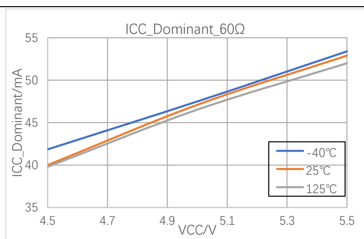
Figure 7-4 Supply Current @ Dominant State ( R_L = 60\Omega )
