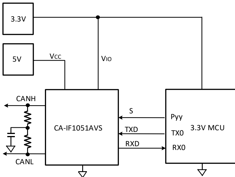
Figure 10- 1 CA-IF1051AVS Typical Application Circuit
