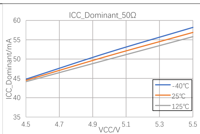
Figure 7-3 Supply Current @ Dominant State ( R_L = 50\Omega )
