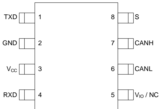
Figure 6-1 CA-IF1051AS/VS Pin Configuration
