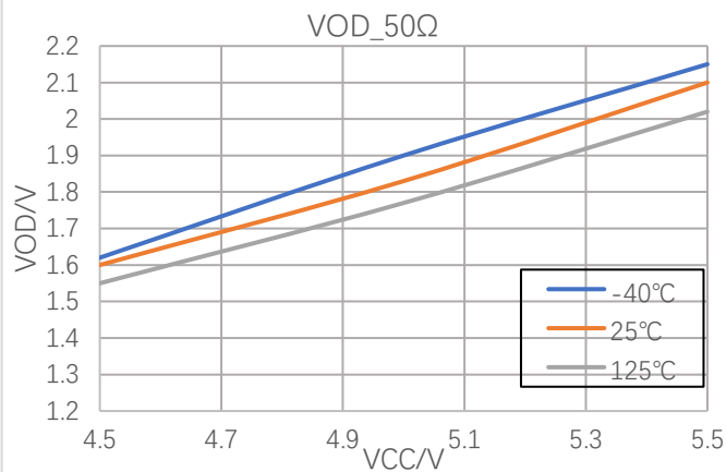
Figure 7-6 Differential Output Voltage vs. V_{CC} ( R_L = 50\Omega )
