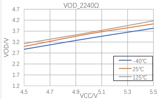
Figure 7-8 Differential Output Voltage vs. V_{CC} ( R_L = 2240\Omega )
