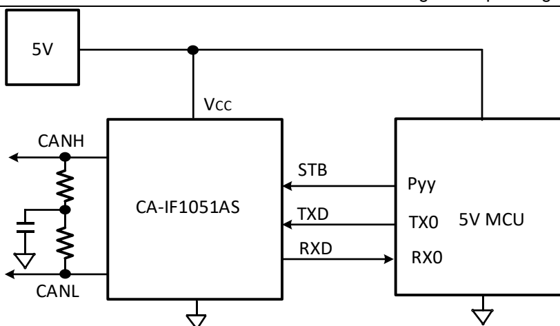
Figure 10- 2 CA-IF1051AS Typical Application Circuit
