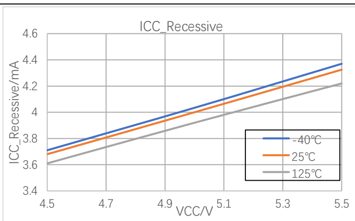
Figure 7-2 Supply Current @ Recessive State
