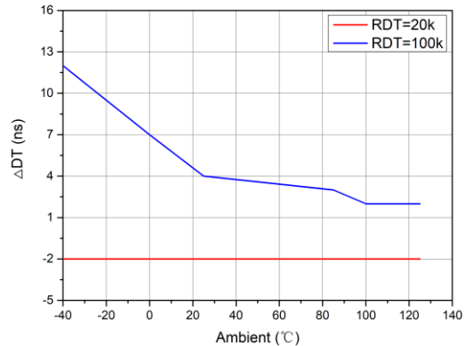
Figure 6-12 Dead time matching vs. Temperature
