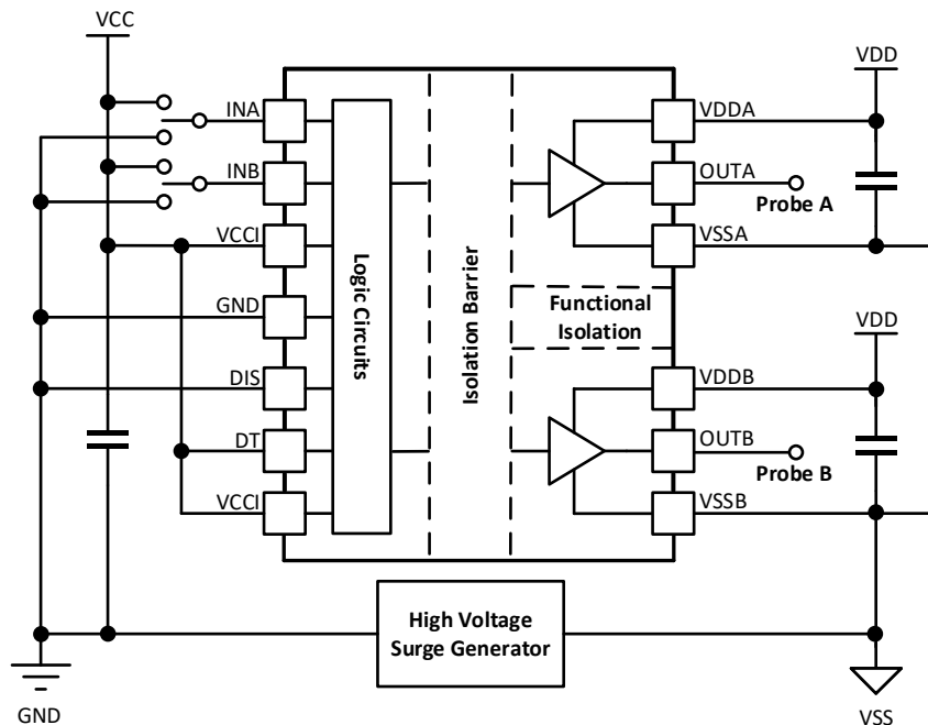
Figure 7-6 Common-mode transient immunity test circuit
