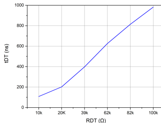
Figure 6-10 RDT vs. Dead time
