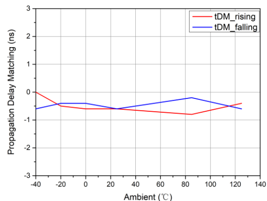
Figure 6-9 Channel delay matching vs. Temperature
