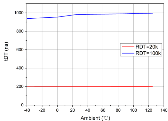
Figure 6-11 Dead time vs. Temperature
