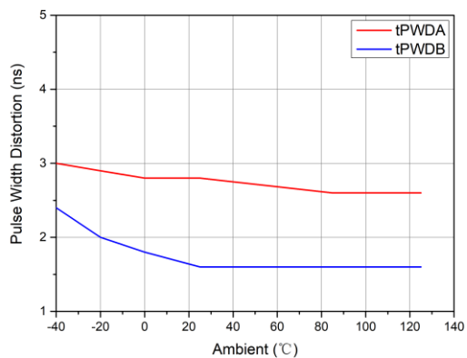
Figure 6-8 Pulse width distortion vs. Temperature
