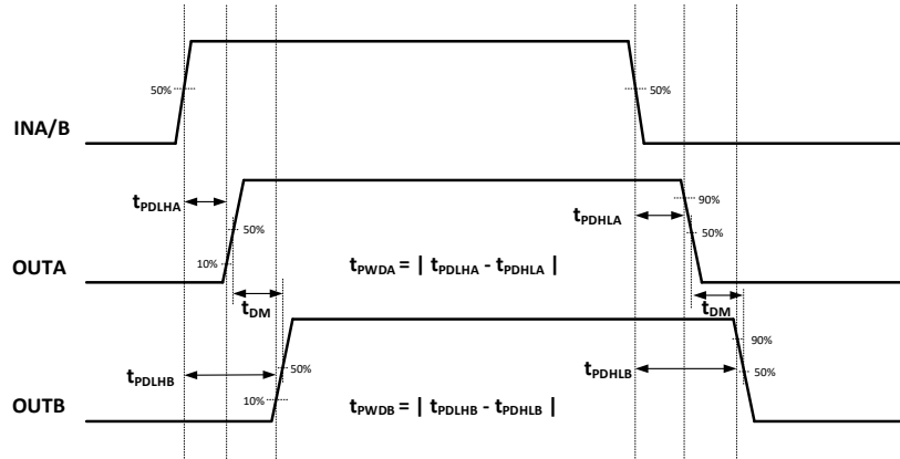
Figure 7-1 Propagation delay and pulse width distortion timing diagram (overlapping input and dead-time disabled)
