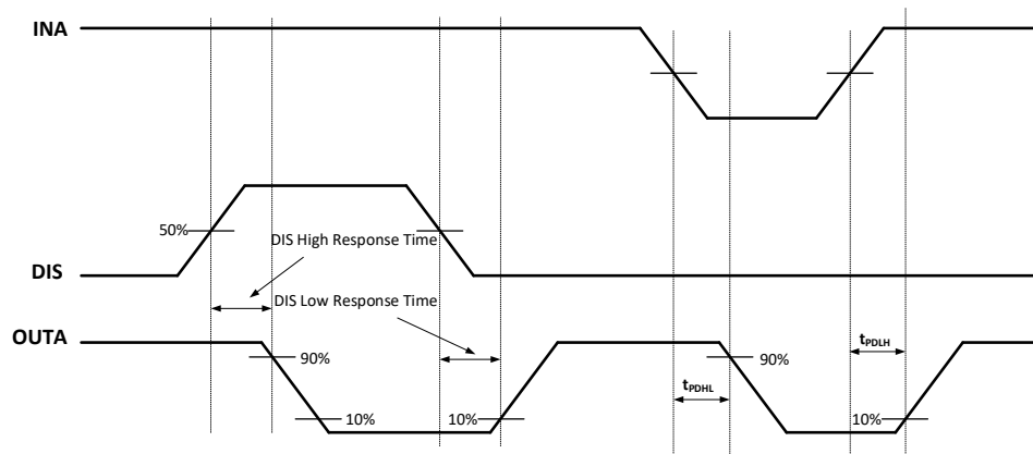
Figure 7-3 Disable timing diagram
