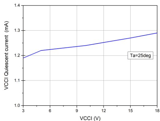
Figure 6-1 VCCI Quiescent current vs. VCCI voltage
