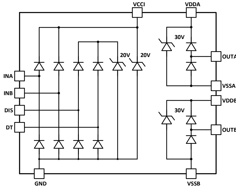
Figure 8-4 ESD protection circuit
