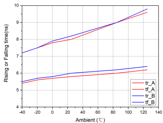
Figure 6-6 Rise time & Fall time vs. Temperature ( C_{load} = 1.8\text{nF} )
