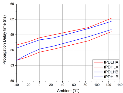
Figure 6-7 Propagation delay time vs. Temperature
