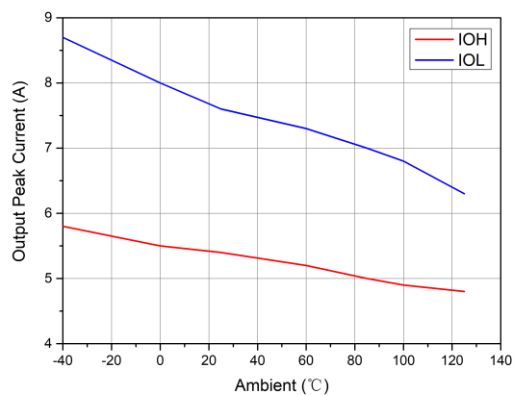
Figure 6-5 Output peak current vs. Temperature ( C_{load} = 180\text{nF} )
