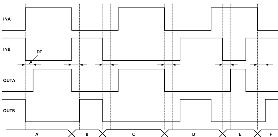
Figure 8-5 Output and input signals relationship with a programmed dead-time
