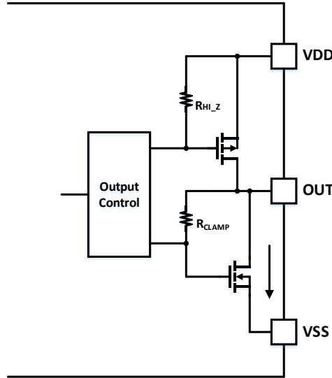
Figure 8-3 Active pull-down
