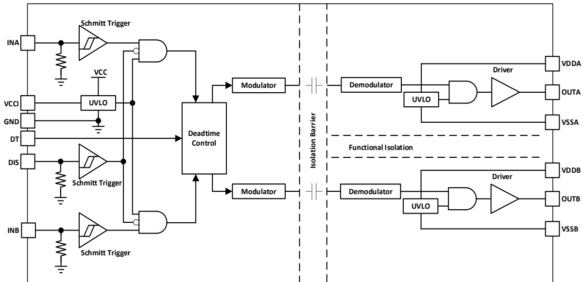
Figure 8-1 Functional block diagram
