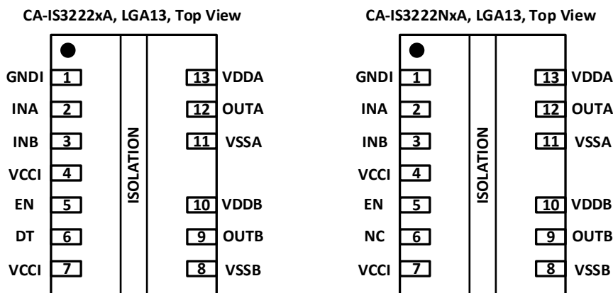
Figure 5-2 The CA-IS3222xA and CA-IS3222Nx A Pin Configuration (LGA13 Package)
