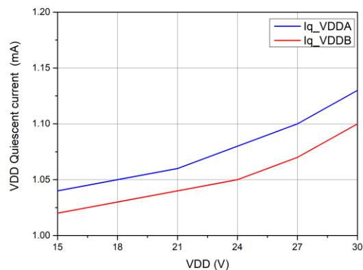
Figure 6-2 VDD Quiescent current vs. VDD voltage
