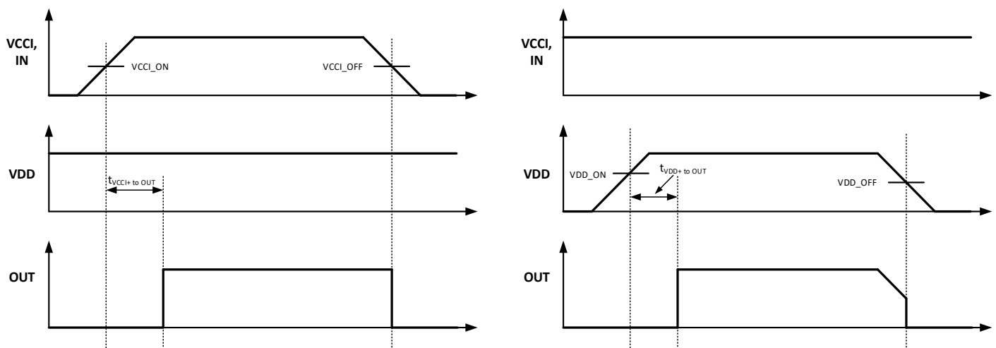
Figure 7-5 VCCI/VDD_ UVLO power-up delay
