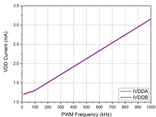
Figure 6-4 VDD operating current vs. PWM frequency (No Load)
