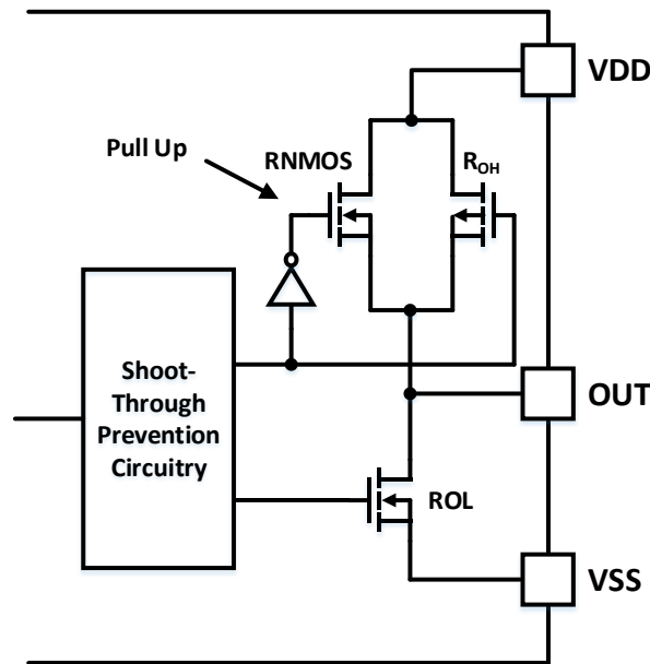
Figure 8-2 Driver output stage
