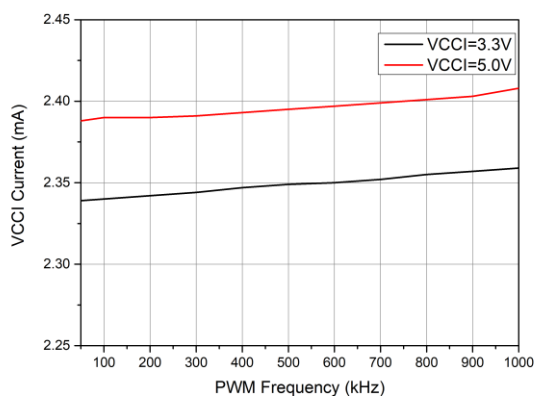
Figure 6-3 VCCI operating current vs. PWM frequency
