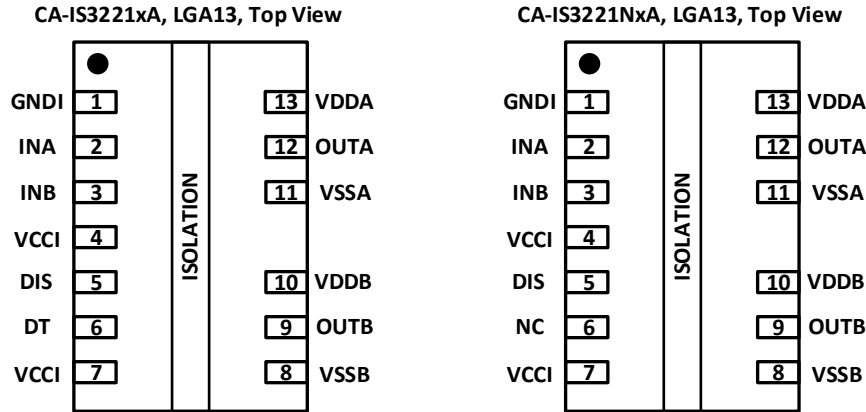
Figure 5-1 The CA-IS3221xA and CA-IS3221Nx A Pin Configuration (LGA13 Package)
