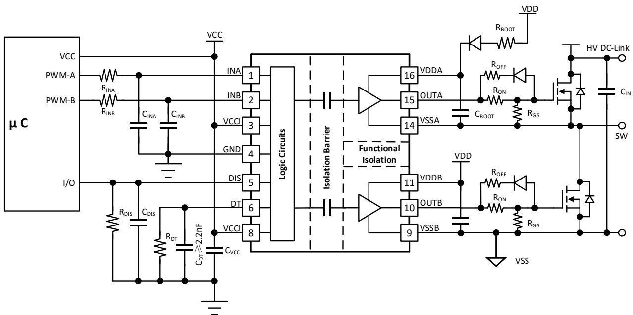
Figure 9-1 Typical application circuit for CA-IS3221
